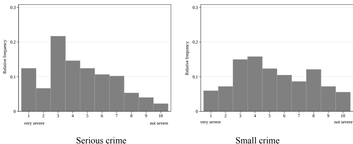
Figure 3. Severity of victimization
