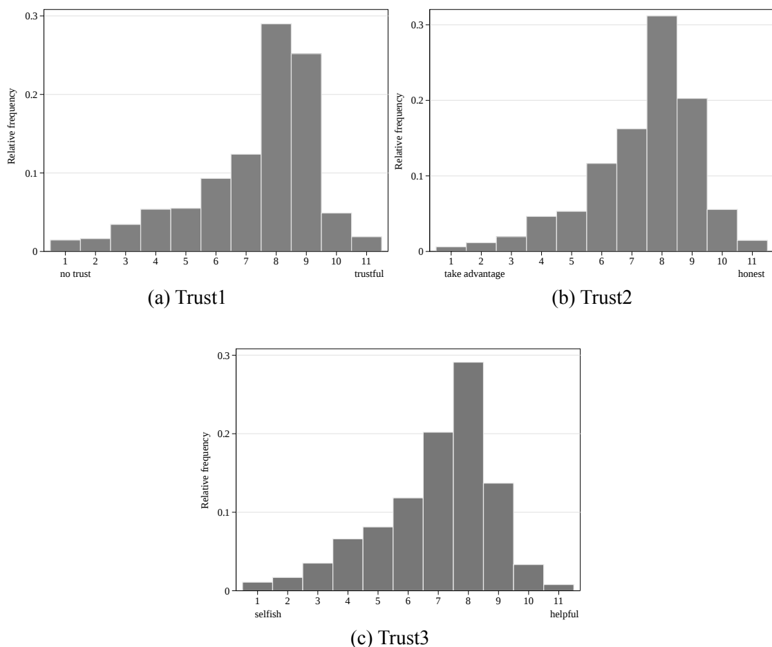
Figure 5. Histograms of trust variables
